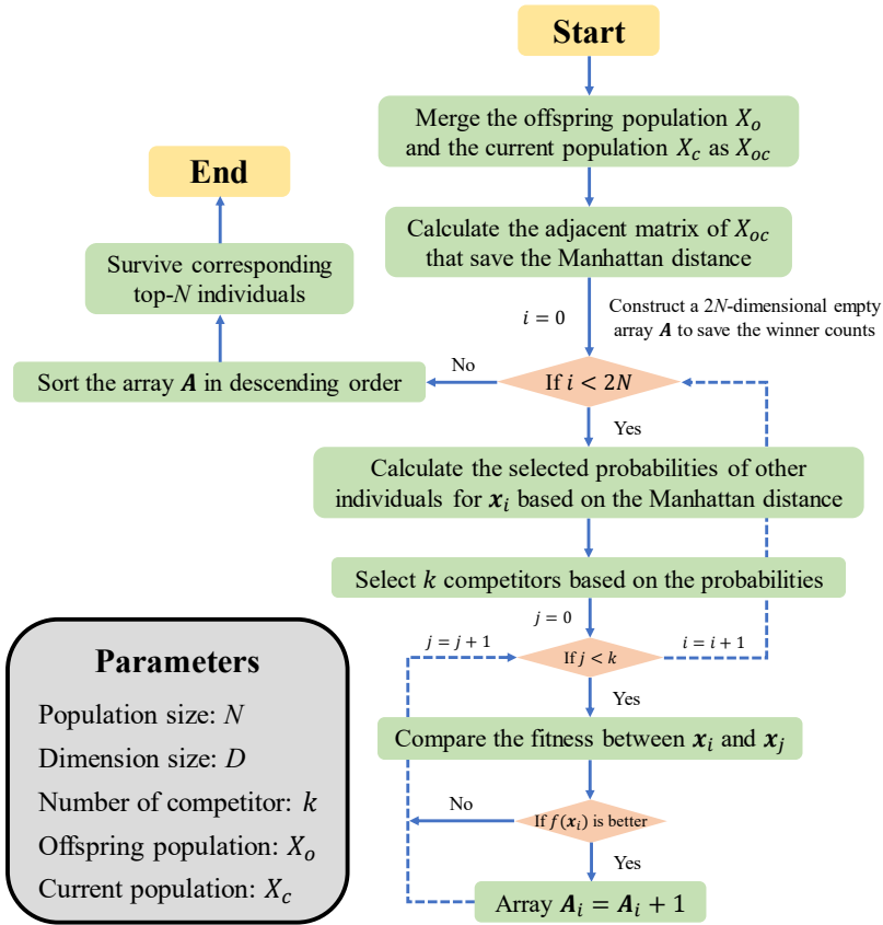
Fig. 1 The flowchart of the AMP selection mechanism.
