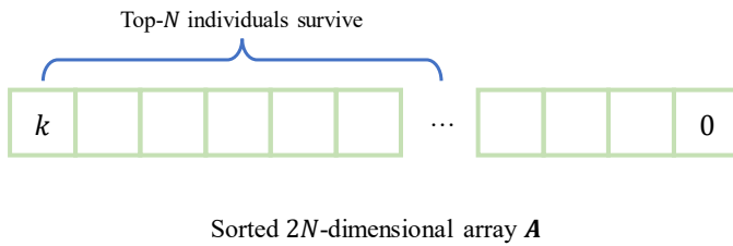
Fig. 3 A demonstration of the top- N selection based on the sorted array \mathbf{A} .
