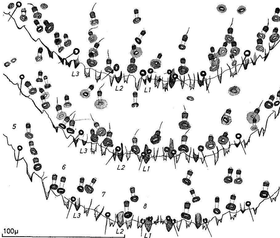
Fig. 5. Aleucaspis salla n. sp. Adult female: pygidial margin in dorsal view. 75NPL-27.
