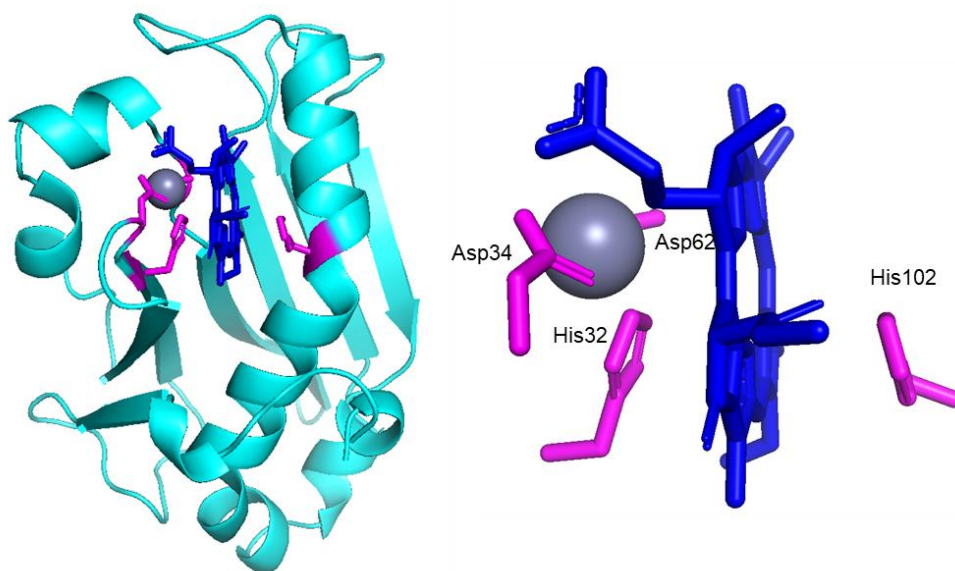
Figure S9. Computational prediction of AbSGR-h, Zn ion, and substrate complex structure.
