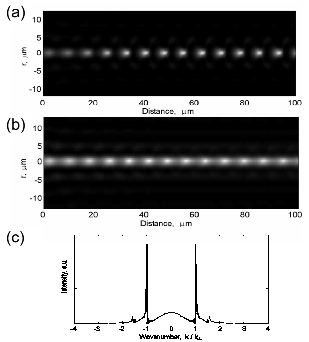
FIG. 2: Instantaneous (at t = 0 in the moving coordinate frame) intensity (a), fluence (b) and the angular spectrum (c) calculated for the GB wave-packet propagating for 100 \mu\text{m} in glass.
