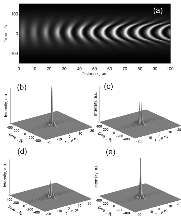
FIG. 1: Calculated zt - image of the on-axis pulse intensity in the moving coordinate frame (above); Below: space-time resolved energy fluence profiles of the wave packets at the distances between z = 50 \mu\text{m} and z = 58.5 \mu\text{m} , representing refocusing cycle of the GB beam in glass.
