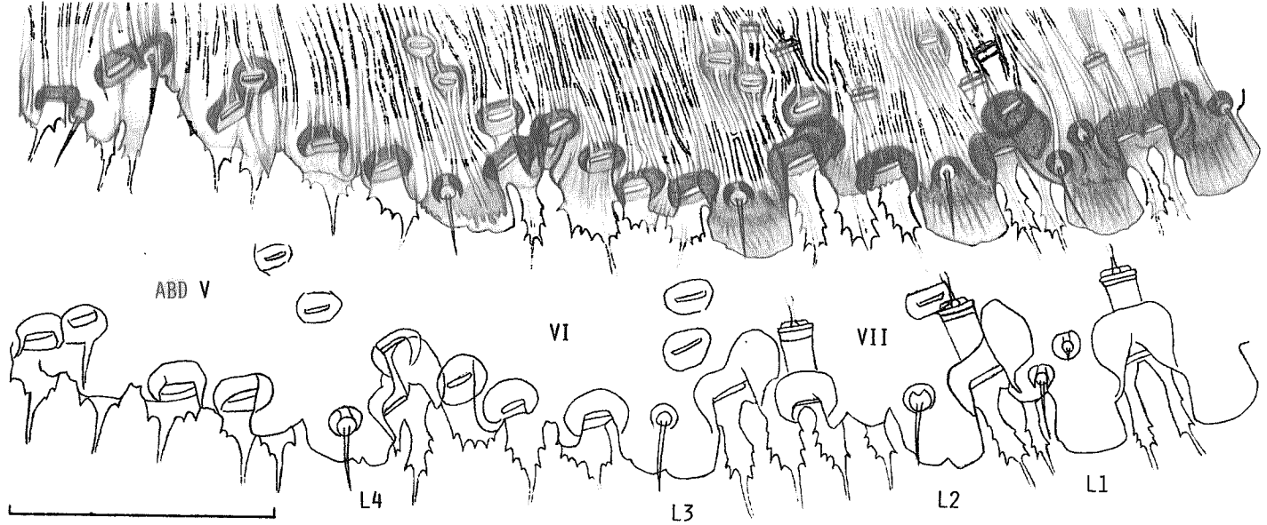
Fig. 11. Tamilparla smilacis , adult female: pygidial margins, dorsal surface. Scale: 0.05 mm.
