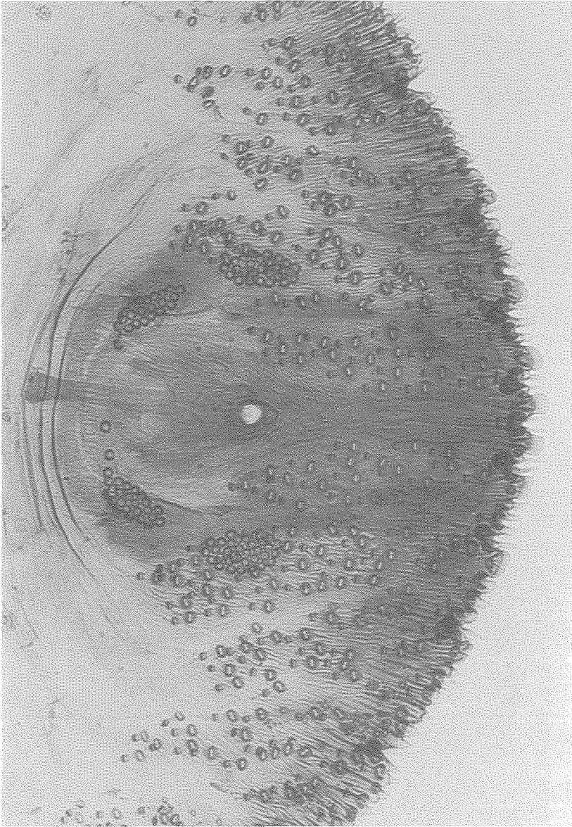
Fig. 9. Tamilparia similis , adult female : pygidium.
