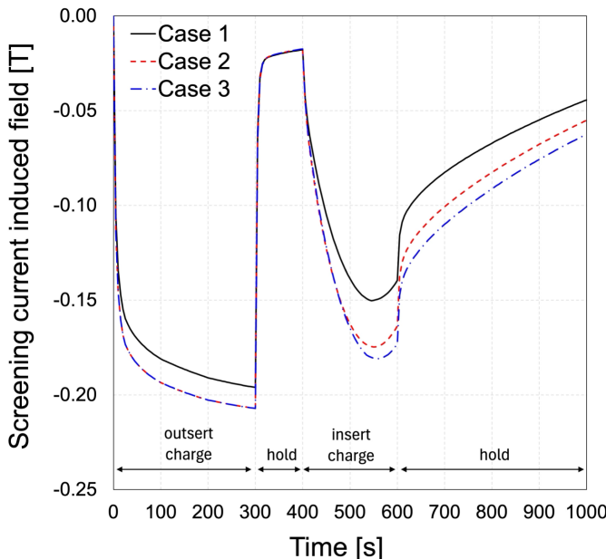
Fig. 7. Screening current induced field during magnet charge. The dummy coil increases the screening current induced field.
