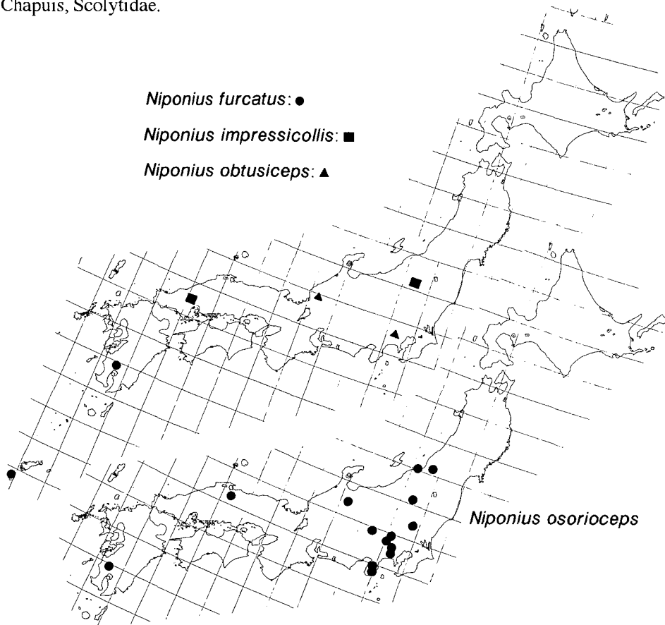
Fig. 48. Collection site of Niponius spp. in Japan.
