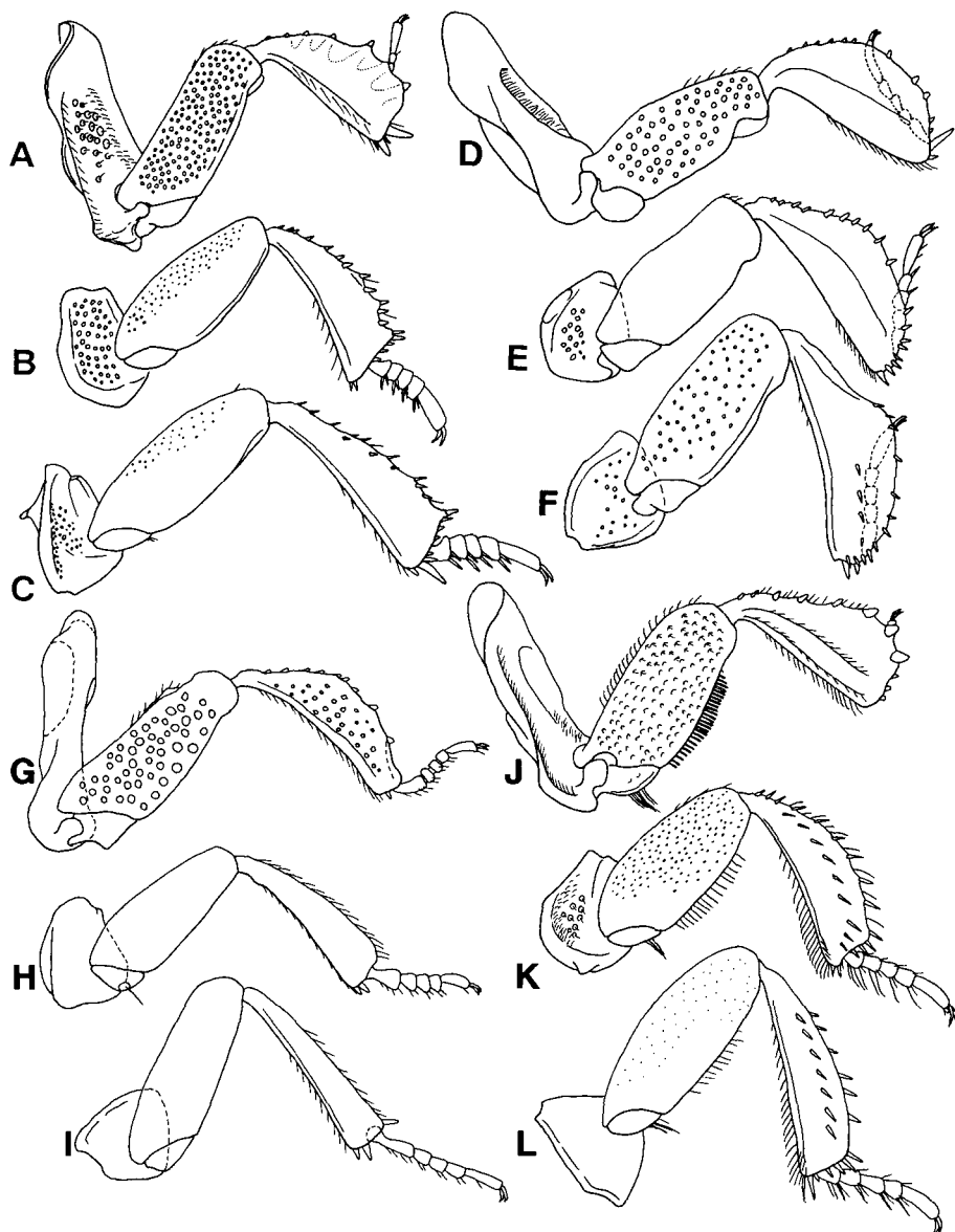
Fig. 30. Legs. A, B, C: Margarinotus cadavericola (Histerini, Histerinae, Histeridae). D, E, F: Dendrophilus xavieri (Dendrophilini, Dendrophilinae). G, H, I: Chaetabraeus bonzicus (Abraeini, Abraeinae). J, K, L: Saprinus splendens (Saprininae). A, D, G, J: Fore legs. B, E, H, K: Mid legs. C, F, I, L: Hind legs.
