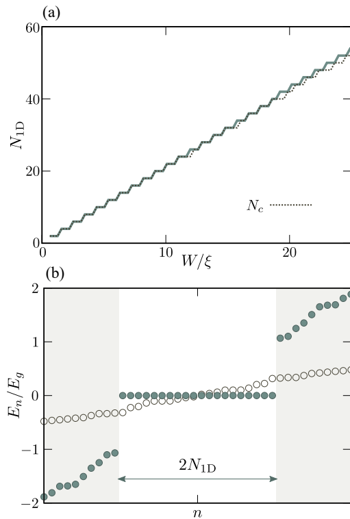
FIG. 2. (a) 1D winding number, N_{1D} , as a function W , with dotted line representing the number of the propagating channels N_c . (b) Energy spectrum under open boundary conditions in both x and y directions, where the colored (white) dots indicate the result for \lambda = 0.5t ( \lambda = 0 ). Each dot corresponds to twofold-degenerate states due to Kramers degeneracy. For \lambda = 0.5t , we clearly observe the emergence of N_{1D} -fold-degenerate ZESs.
