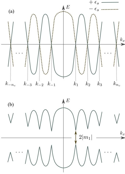
FIG. 4. Schematic of the energy spectra of the ABSs for (a) \tilde{\lambda} = 0 and for (b) \tilde{\lambda} \neq 0 , described by the effective Hamiltonian in Eq. (13).
