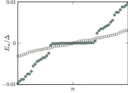
FIG. 6. Energy spectrum of the full Hamiltonian, where the colored (white) dots indicate the result for \lambda = 0.5t ( \lambda = 0 ). Each dot corresponds to twofold-degenerate states due to Kramers degeneracy. For \lambda = 0.5t , we clearly observe the emergence of highly degenerate zero-energy states.
