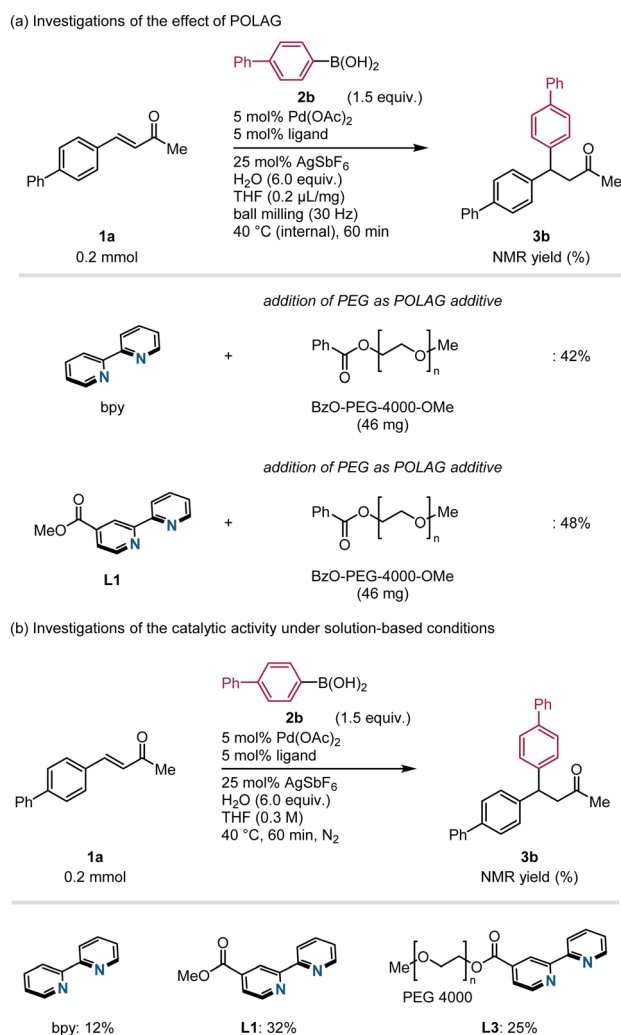
Scheme 5 Control experiments.
