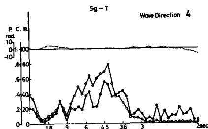
Fig. 16. The response characteristic and coherency between the surging motion and the warp tension in wave scale 3 (wave direction 4, See Fig. 10 for wave direction 1).
