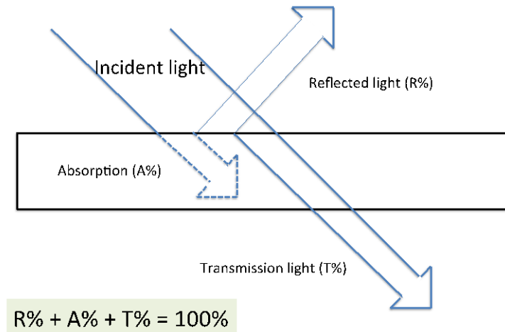
Fig. 2-20 Simple model of incident light passing through a plastic sample
