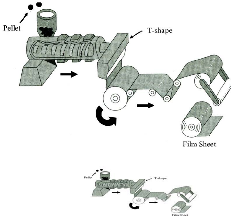
Fig. 2-6 T-die method to fabricate plastic films
