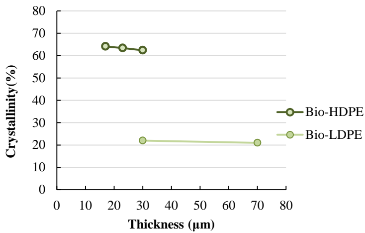
Fig. 2-7 Crystallinity of bio-based PE
