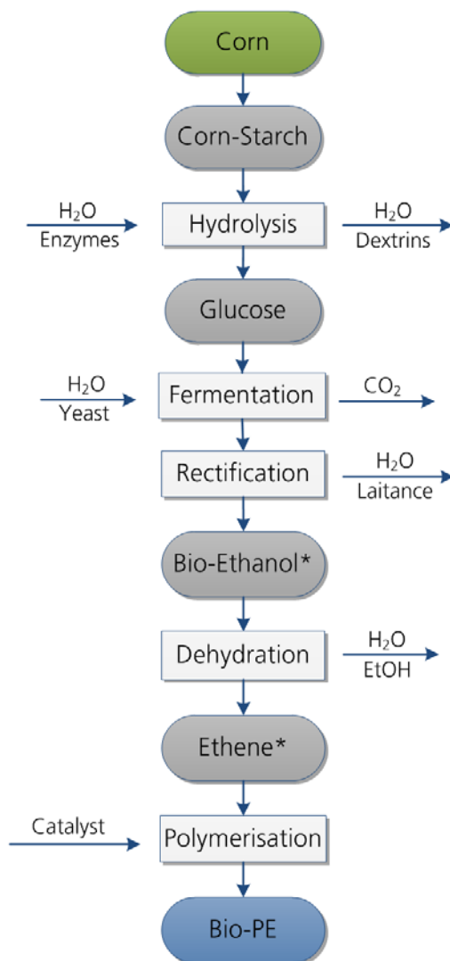
Fig. 1-6 Produce processing of bio-based Polyethylene
