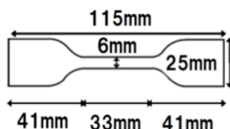
Fig. 2-11 A sketch of dumbbell shaped film sample having dimensions according to JIS K7113 No. 2, JIS K7127 type 5 for measuring mechanical properties
