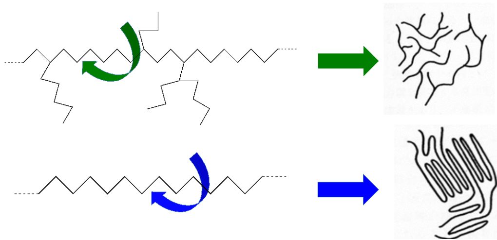
Fig. 2-8 Model of molecular chains of LDPE (upper) and HDPE (lower)
