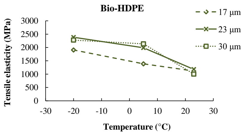
Fig. 2-13 Temperature affected tensile elasticity
