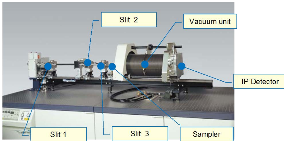
Fig. 2-3 Wide-angle X-ray Scattering (WAXS)
