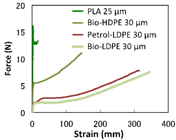
Fig. 2-12 Force-strain curves of plastic samples
