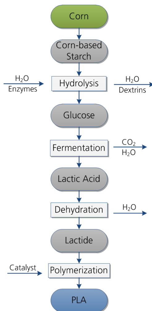
Fig. 1-3 Produce processing of PLA (from Institute for Bioplastics and Biocomposites)
