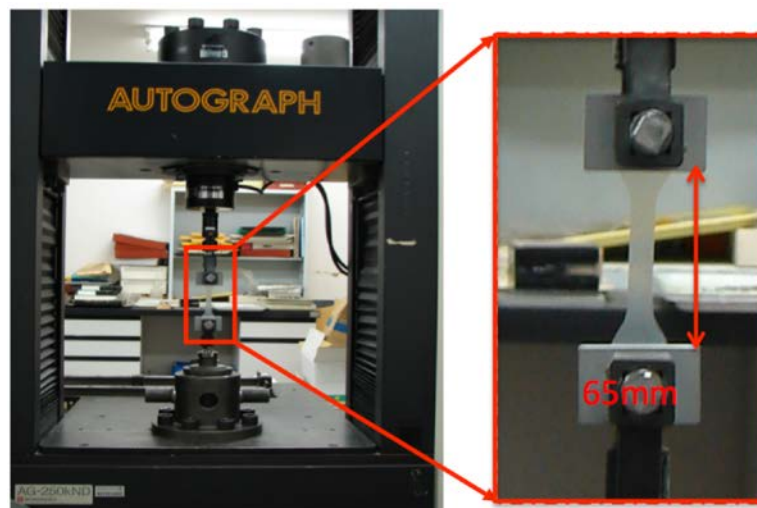
Fig. 2-10 Universal testing machine system (model AG-250kND, Shimadzu, Japan) for measuring mechanical properties
