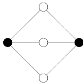
K_{2,3}
