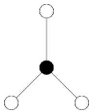
K_{1,3}
