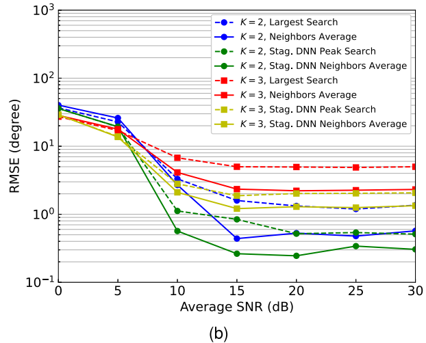
Fig. 7 Estimation accuracy improvement by the proposed technique named “Neighbors Average”. (a) Probability of correct DOA estimation. (b) RMSE.
