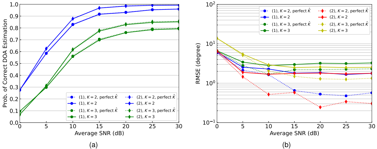
Fig. 11 Proposed system performance comparison when source number estimation is perfect ( \hat{K} ) and not perfect, and when SNR-based (1) Switching DNN or (2) Switching Staggered DNNs are used as spectrum estimation techniques. SNR estimation is done with the regression-based method. (a) Probability of correct DOA estimation. (b) RMSE.
